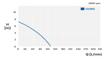
HV180-AV with a vertical magnetic switch
